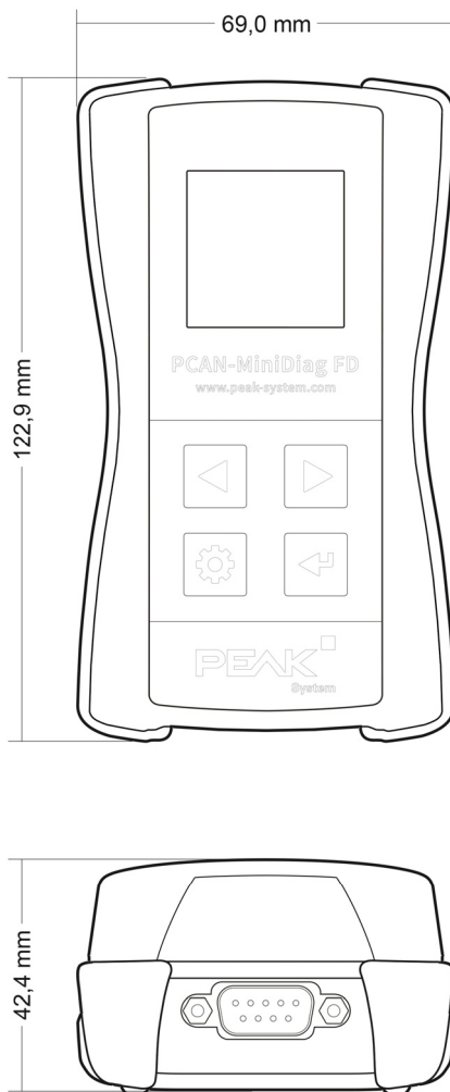
Figure 21: Dimension drawing of the PCAN-MiniDiag FD. The figure does not correspond to the actual size.
