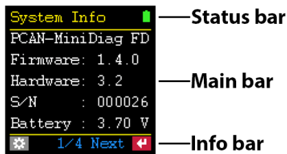
Figure 2: Display structure
