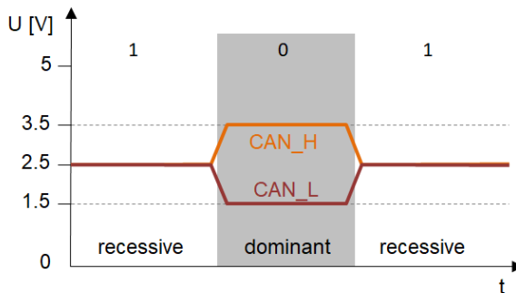
Figure 22: Diagram of the recessive and dominant signal levels on the CAN bus
