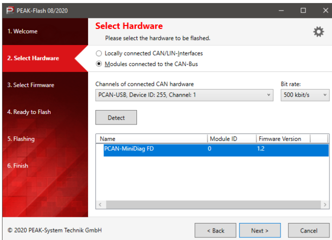
Figure 19: Hardware selection
