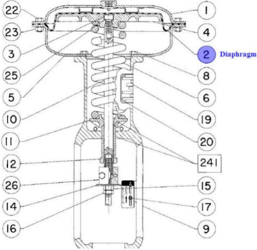
"FISHER" Type 657 Diaphragm Actuator
